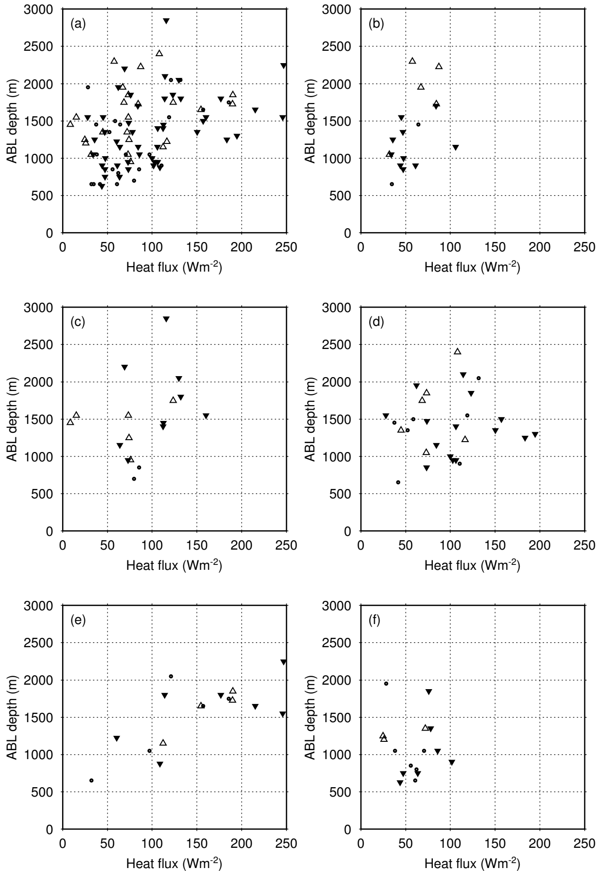
Figure 9 850hPa Relationship between Flux and ABL depth, Shouxian, China, LAPS Hiroki TANAKA
