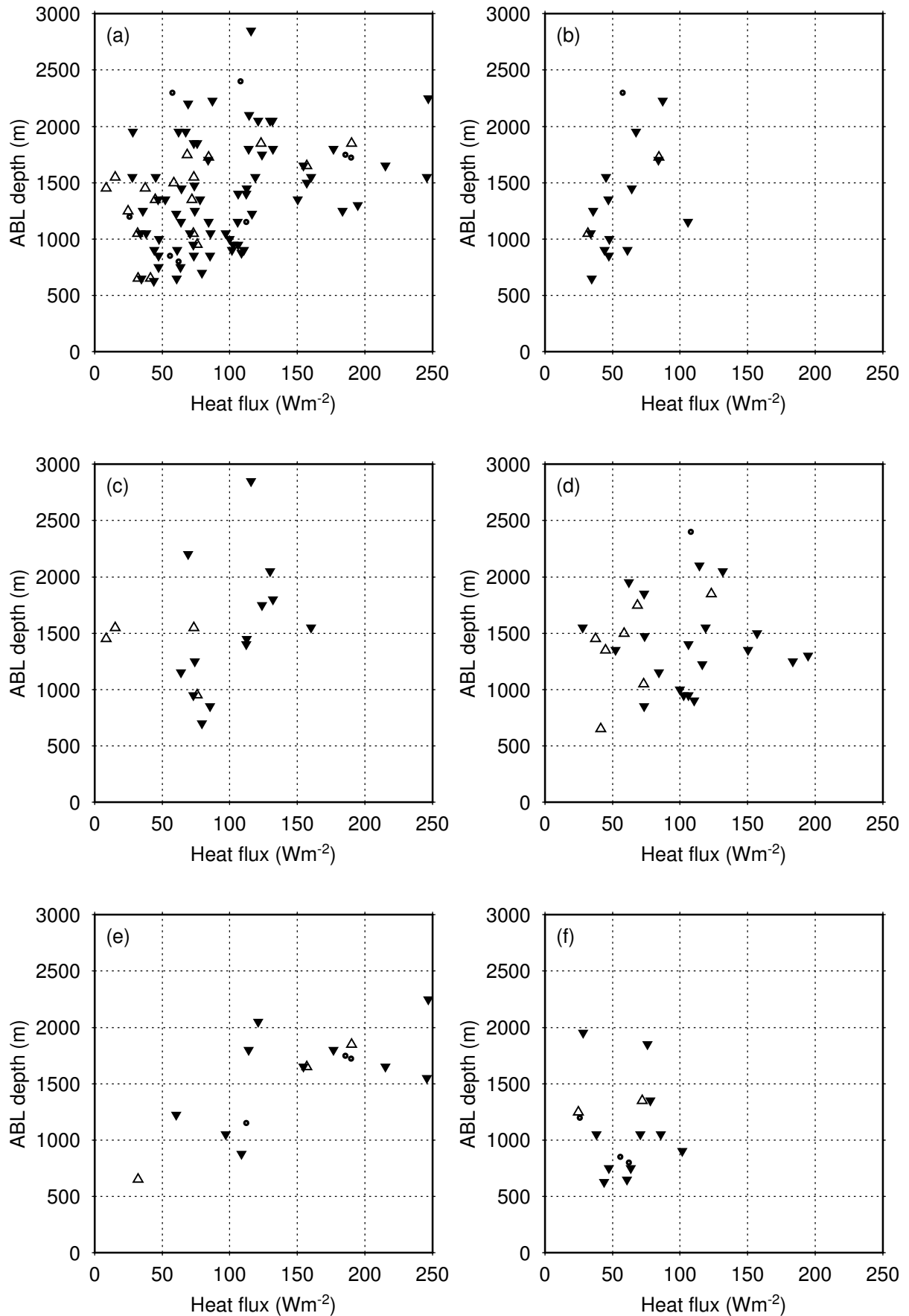
Figure 9 700hPa Relationship between Flux and ABL depth, Shouxian, China, LAPS Hiroki TANAKA
